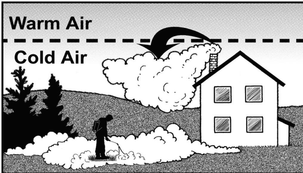
Figure 8-2: Temperature inversion.
