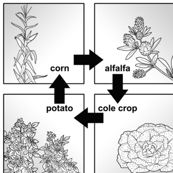
Figure 3-8: Crop Rotation
