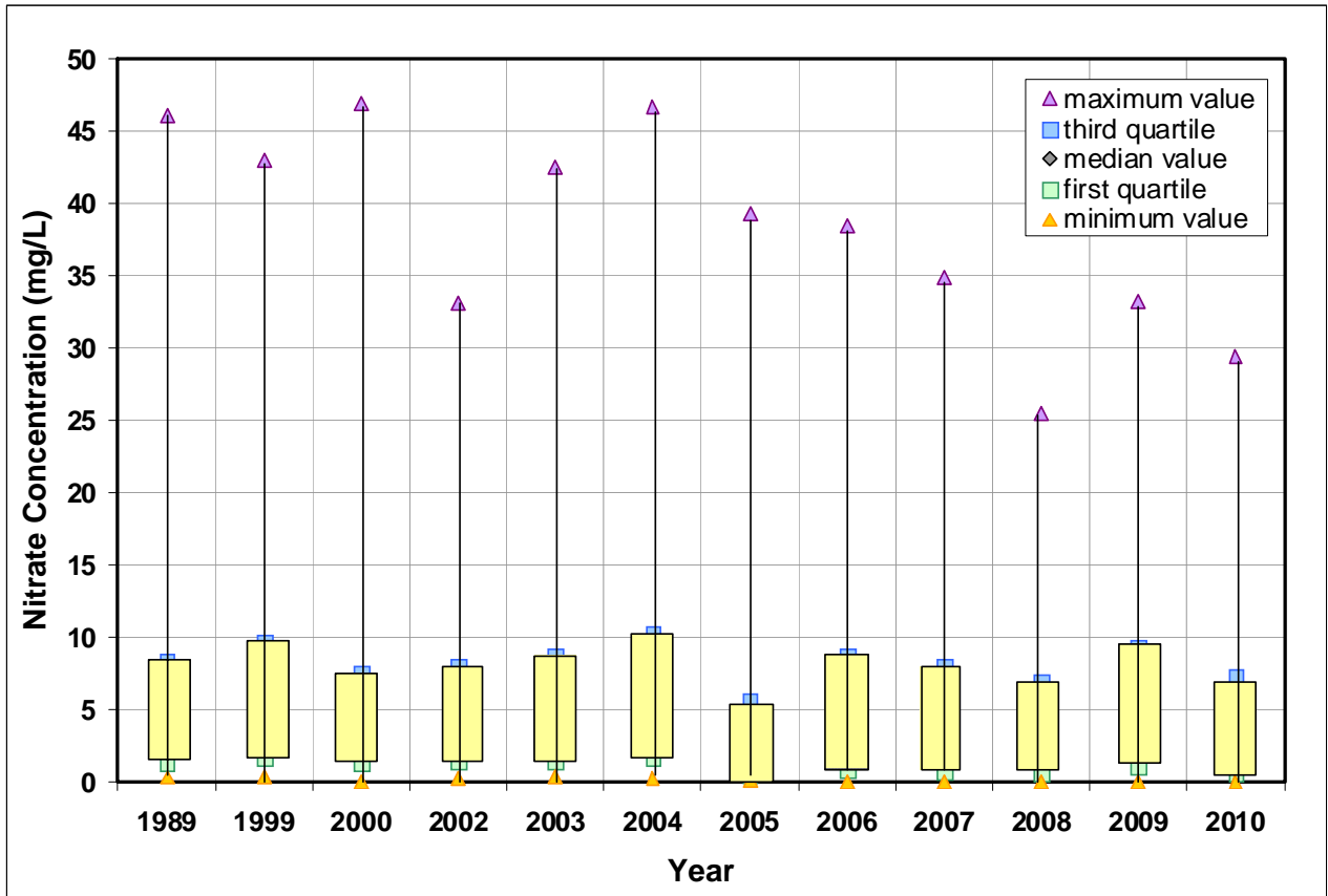
Figure 3-1: Box-Whisker Plots of Nitrate Concentrations in Well Water (1989 - 2010)
