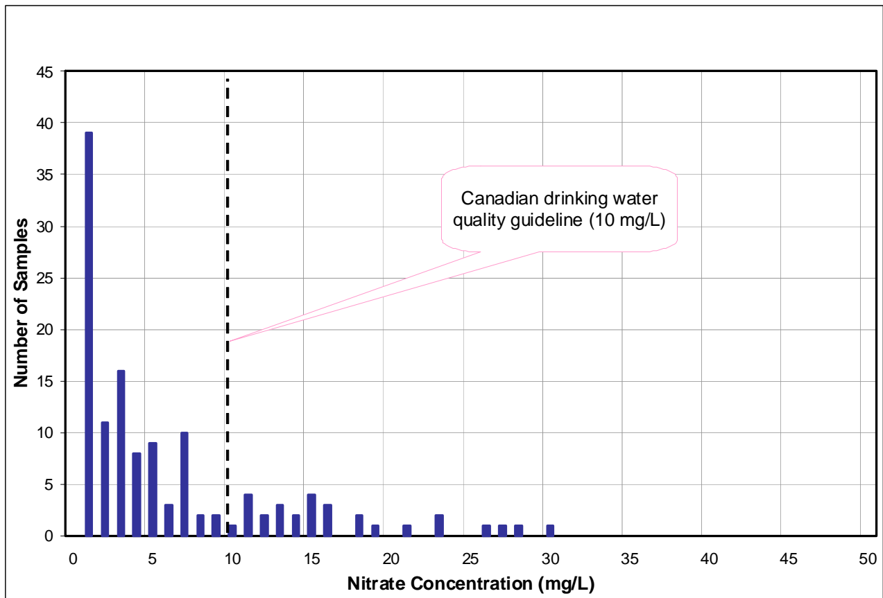
Figure 3-3: Summary of Nitrate Concentrations in Well Water for 2010
