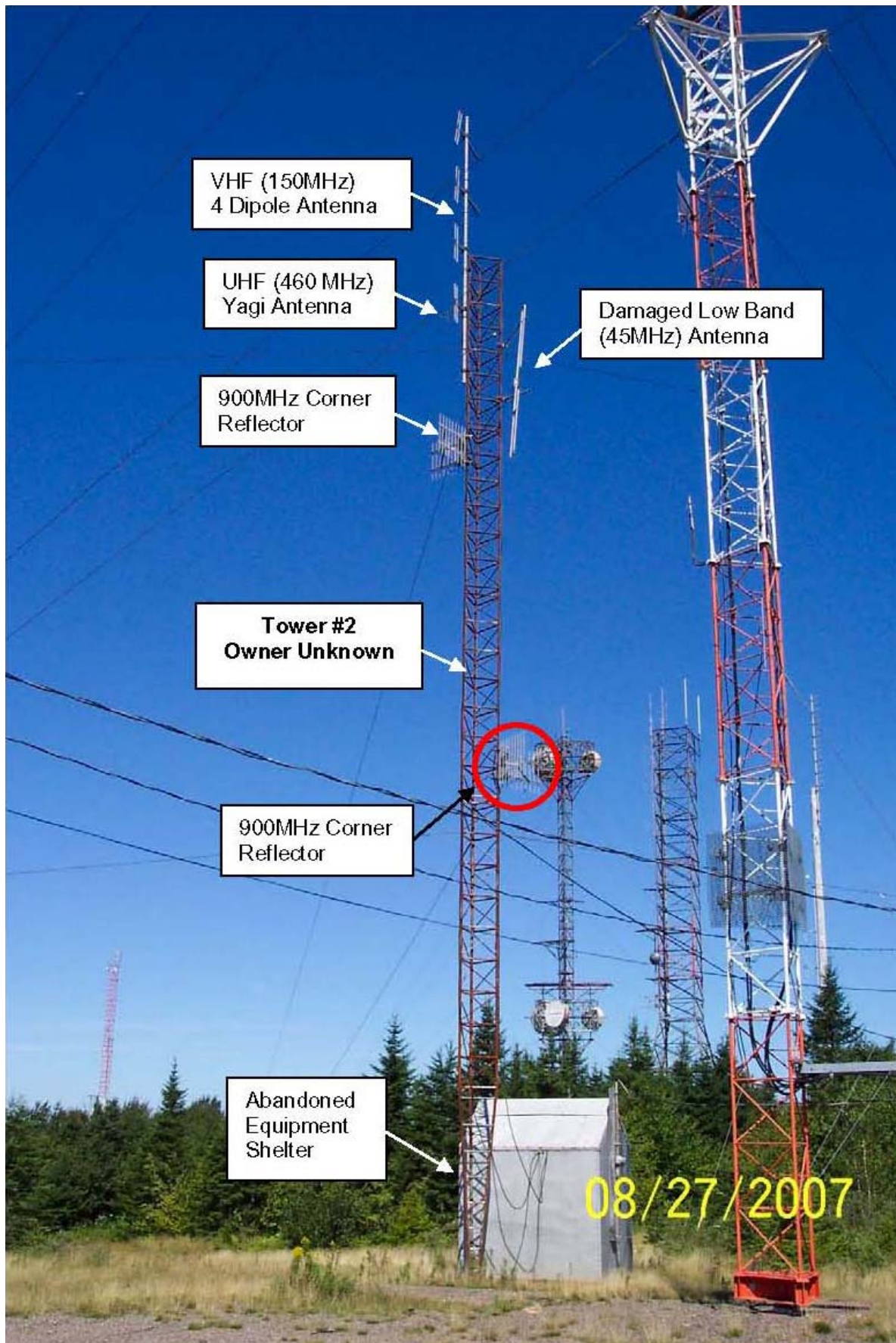
Tower #2 Antenna Inventory
