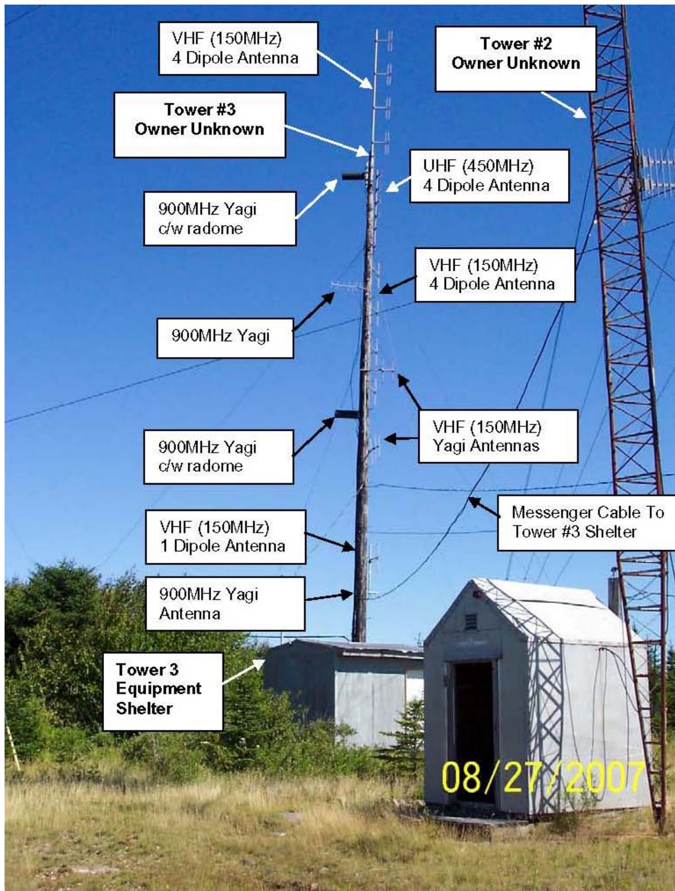
Tower #3 Antenna Inventory
