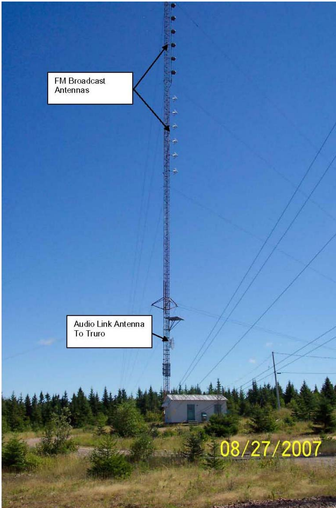
Tower #10 - Broadcast
