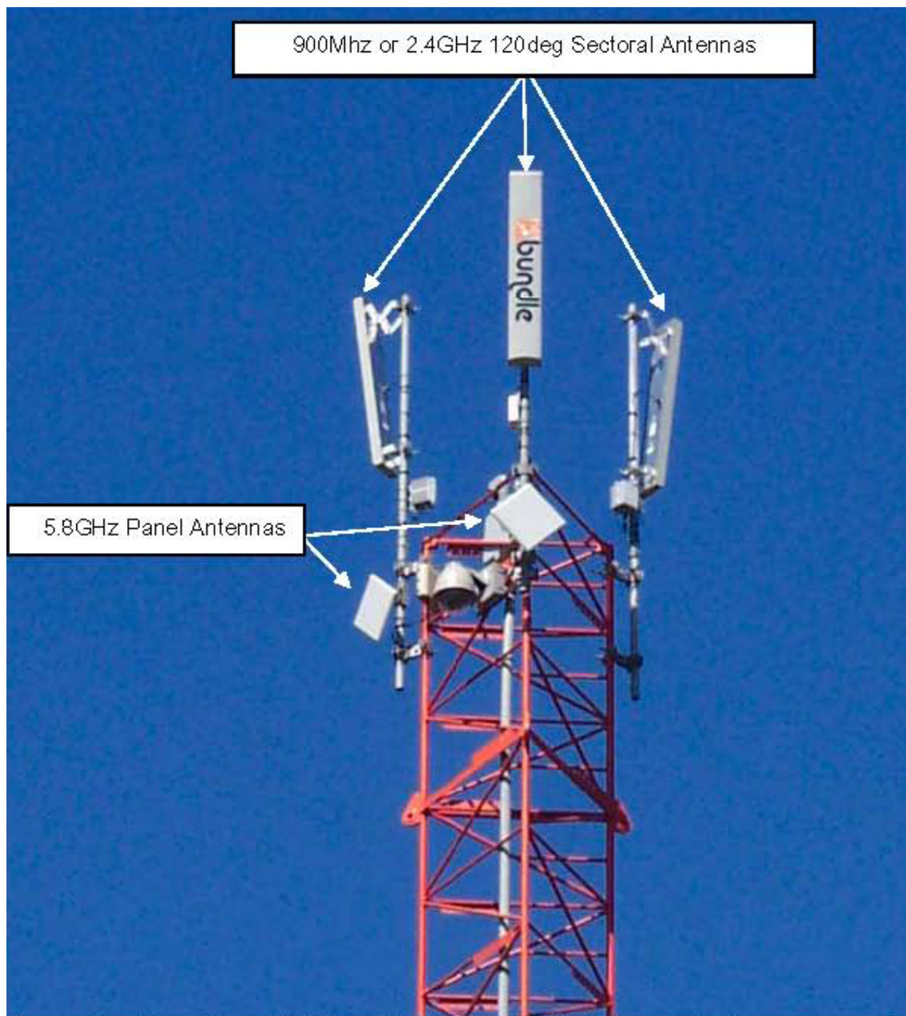
Close Up of NetBundle Wireless INet Antenna System
