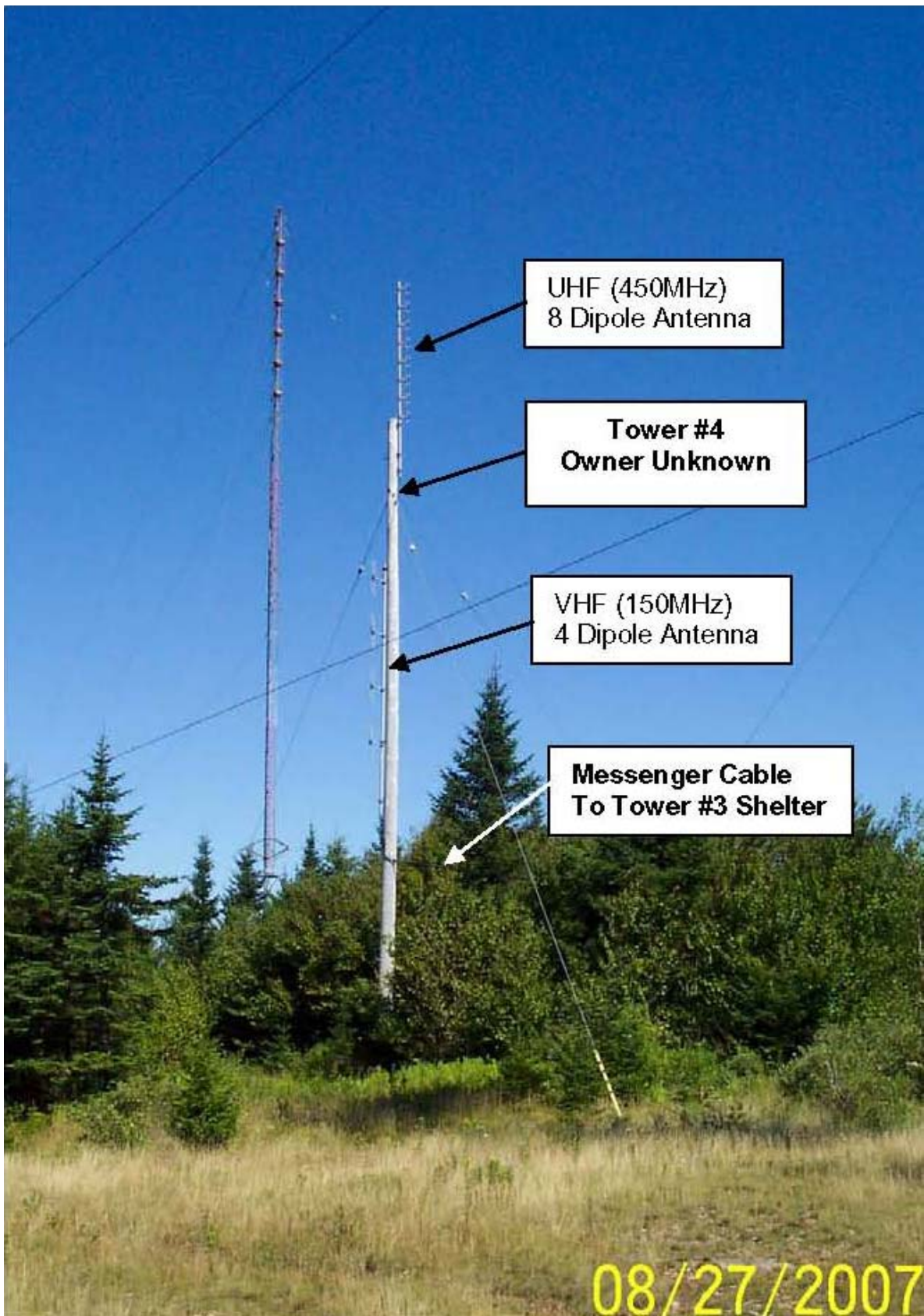
Tower #4 Antenna Inventory
