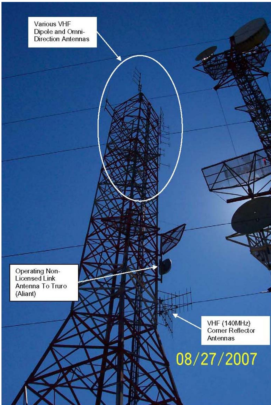
Tower #9 (Aliant) – Antenna Inventory
