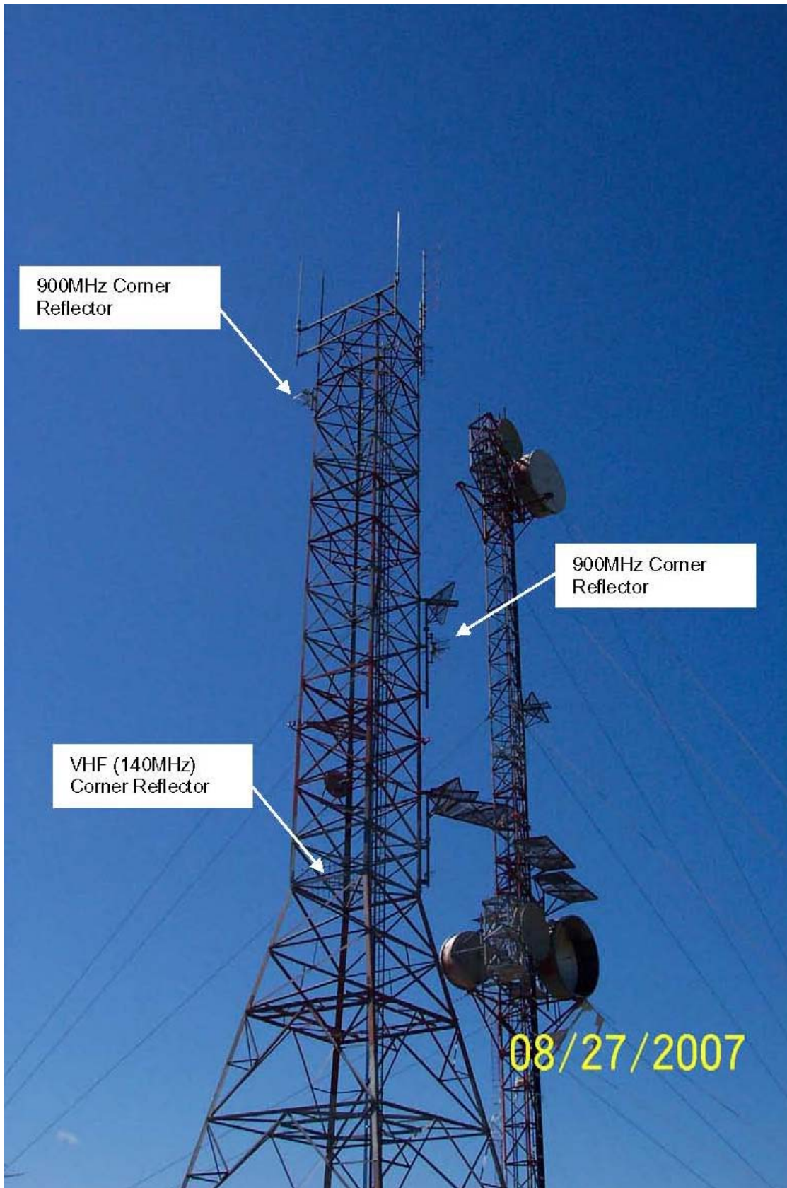
Tower #9 (Aliant) – Corner Reflector Antennas
