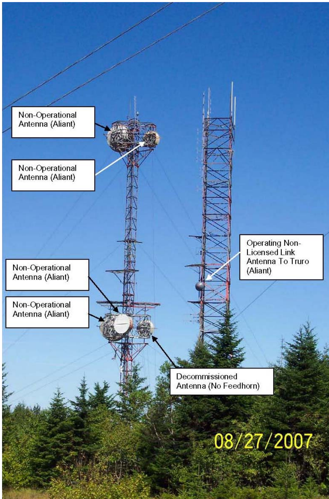
Tower #8 and Tower #9 (Aliant) – Parabolic Antenna Inventory
