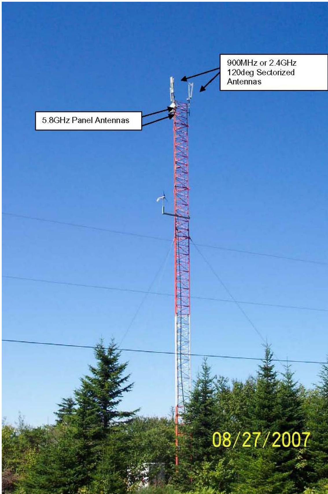
Tower #7 (NetBundle) Antenna Inventory
