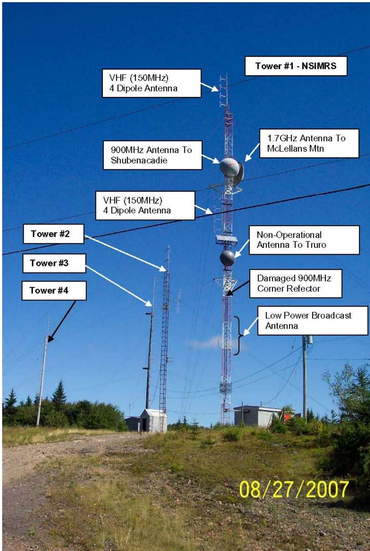
Tower #1 NSIMRS Antenna Inventory
