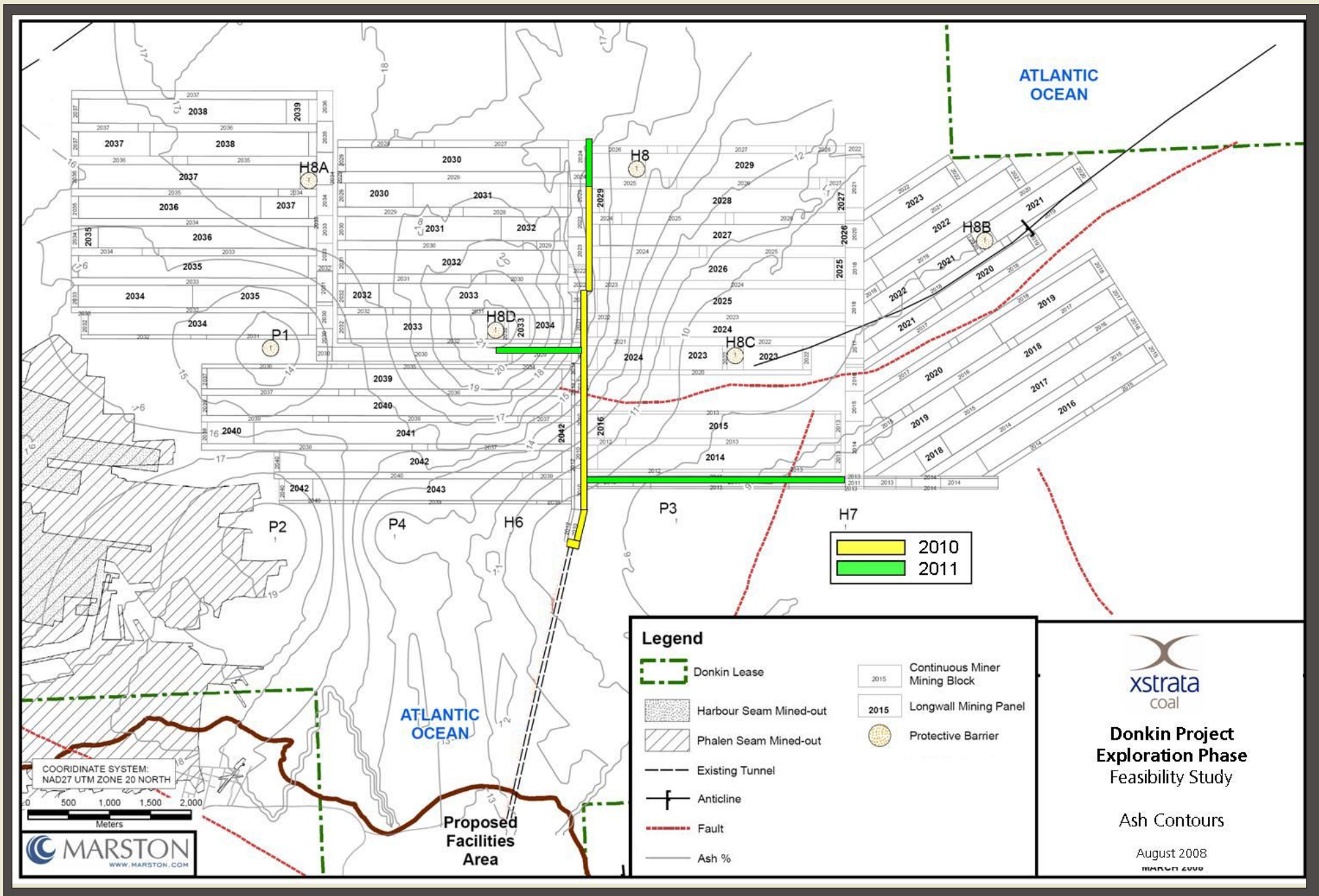
FIGURE 2.1: Underground Exploration Plan (2010 / 2011)
