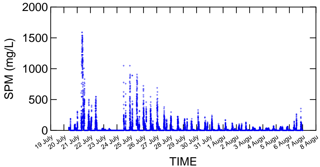
Figure 2.20. Suspended sediment concentrations (SPM) at CYCLOPS 2, 20 July -7 August, 2002.
