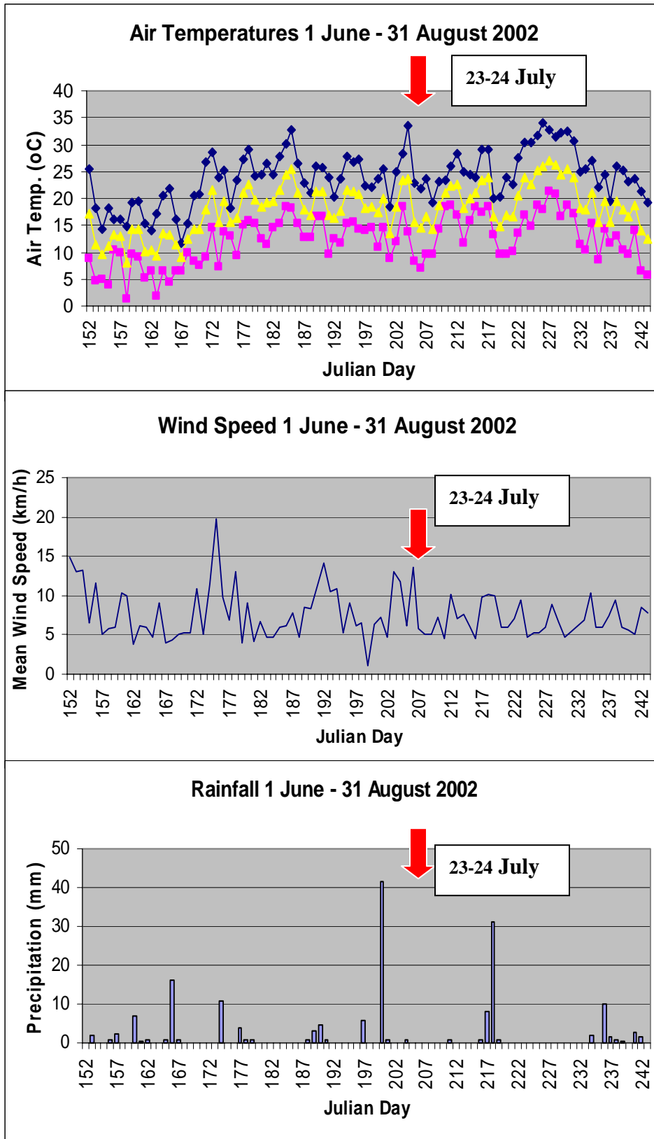
Appendix 2. Weather data for Kentville, 1 June-31 August 2002.
