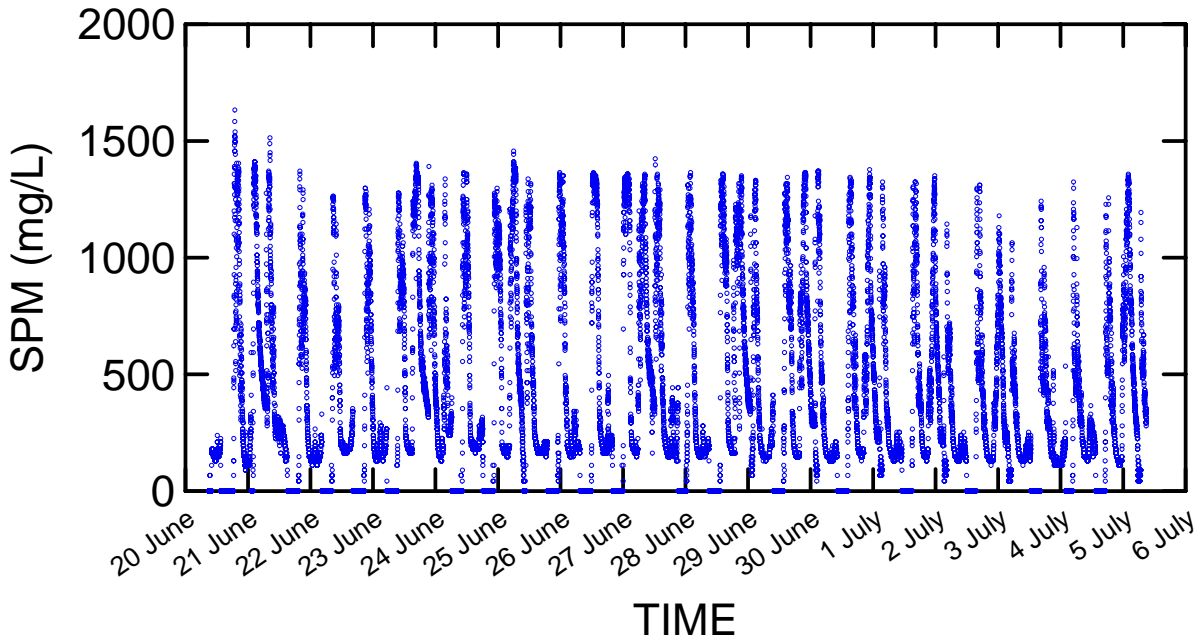
Figure 2.16. Suspended sediment concentrations (SPM) at CYCLOPS 1, 20 June -5 July 2002.
