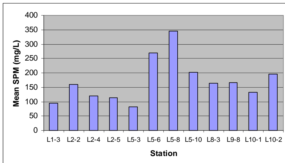
Figure 2.15 Mean suspended sediment concentrations of flood water, 23-24 July 2002.
