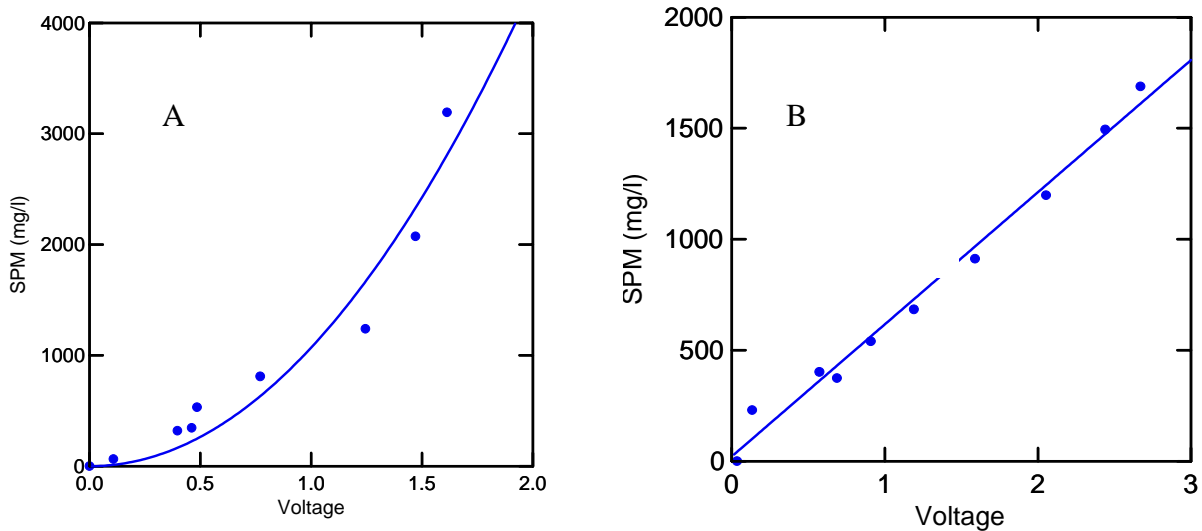
Figure 2.3 Calibration curves for OBS sensors on A. CYCLOPS, B. EMP 2000.
